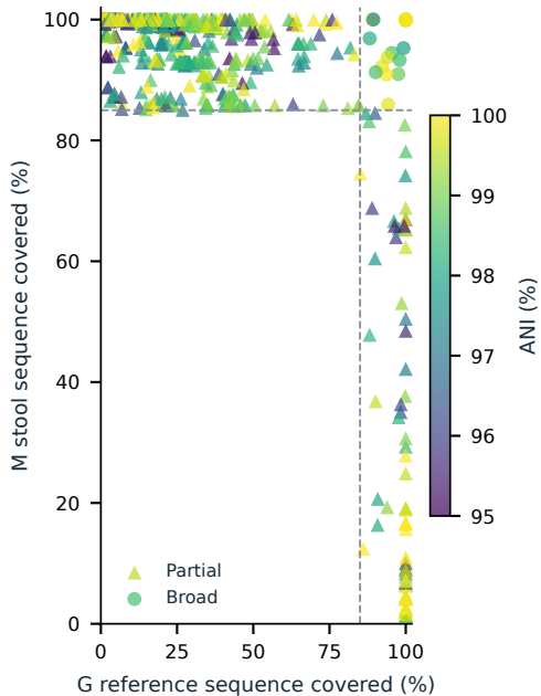
a Direct G-M sequence evidence
