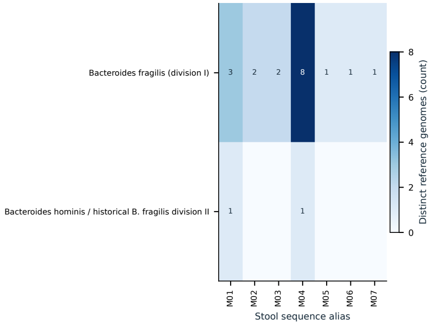
b Reference links for stool sequences
