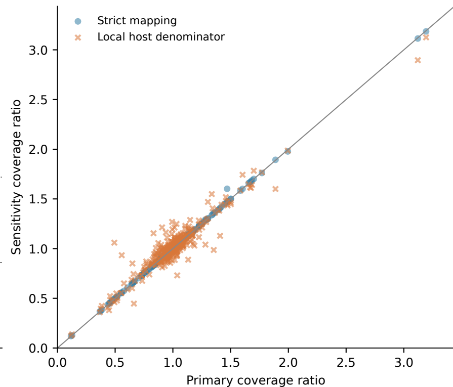
C Finite method sensitivity
