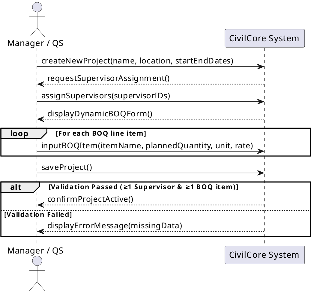
ssd-UC-02.svg: Setup Project and Manual BOQ Entry
