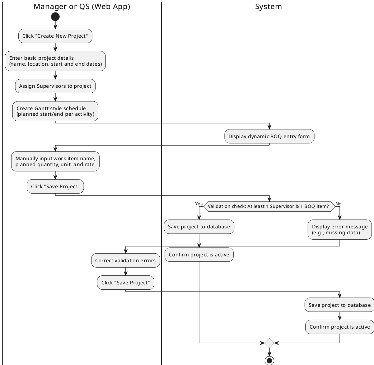
Activity Diagram: UC-02 Setup Project and Manual BOQ Entry
