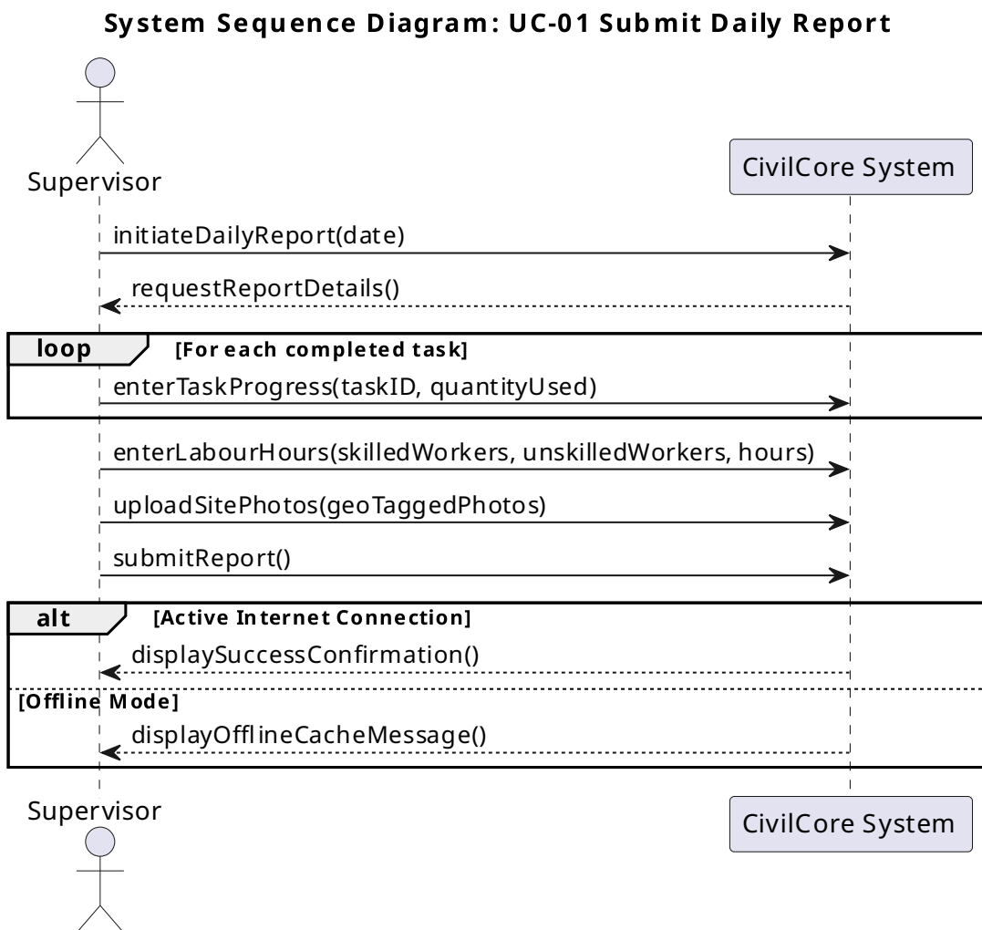
ssd-UC-01.svg: Submit Daily Report
