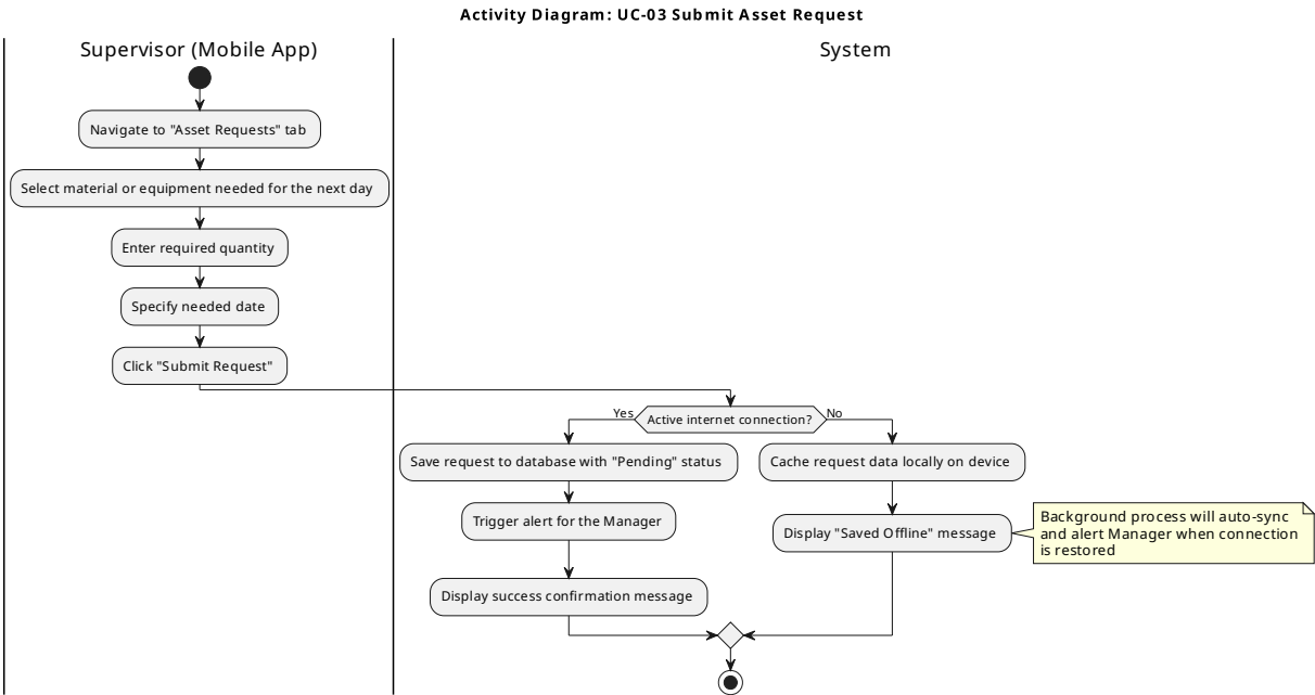
act-UC-03.svg: Submit Asset Request
