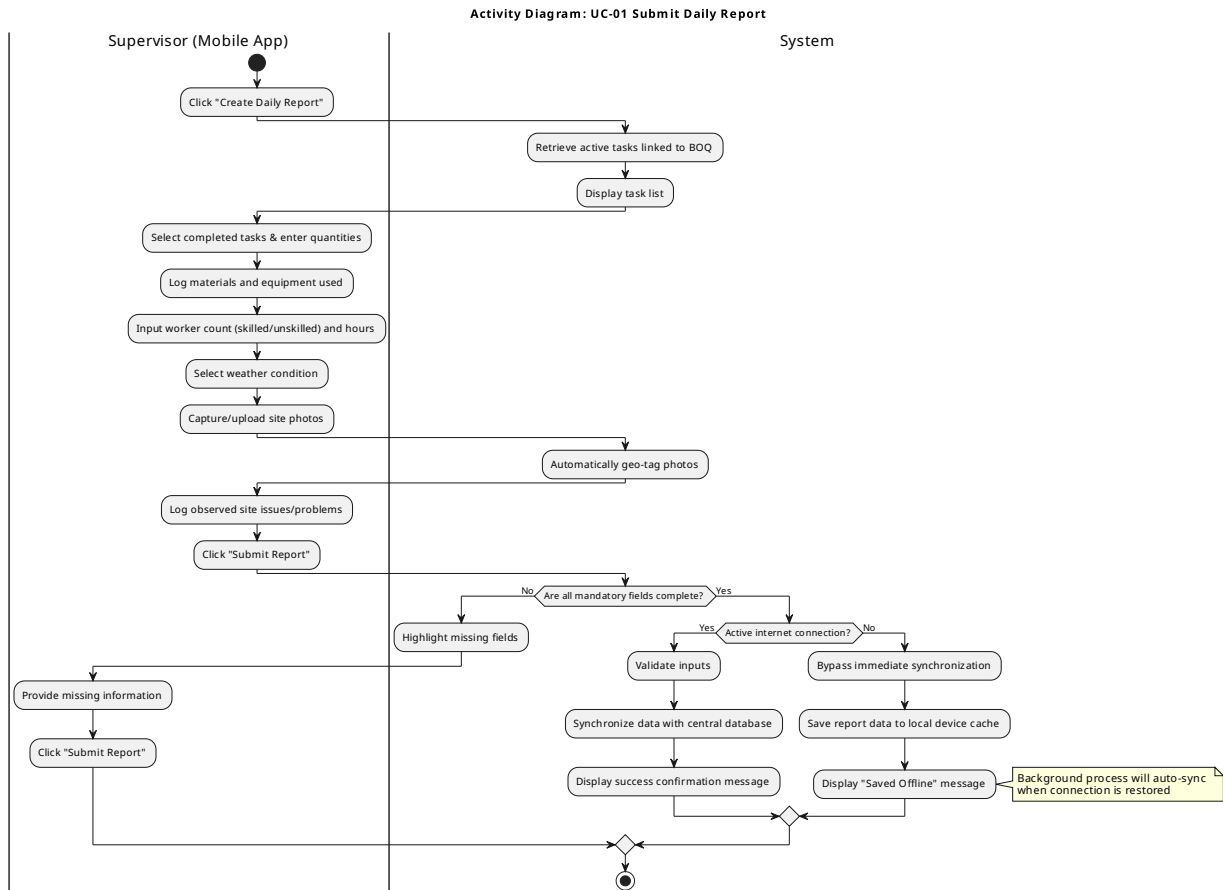
act-UC-01.svg: Submit Daily Report
