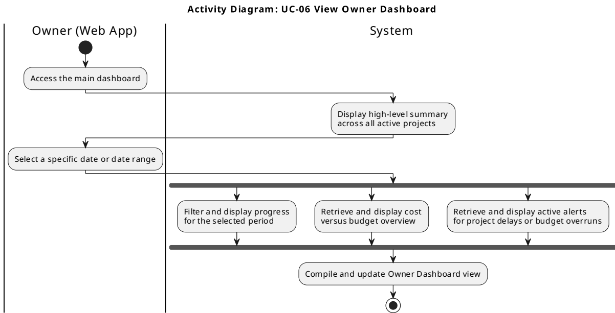
act-UC-06.svg: View Owner Dashboard
