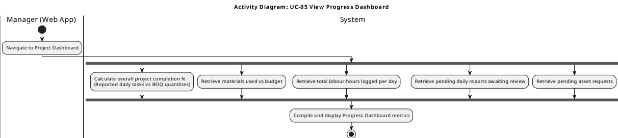
act-UC-05.svg: View Progress Dashboard
