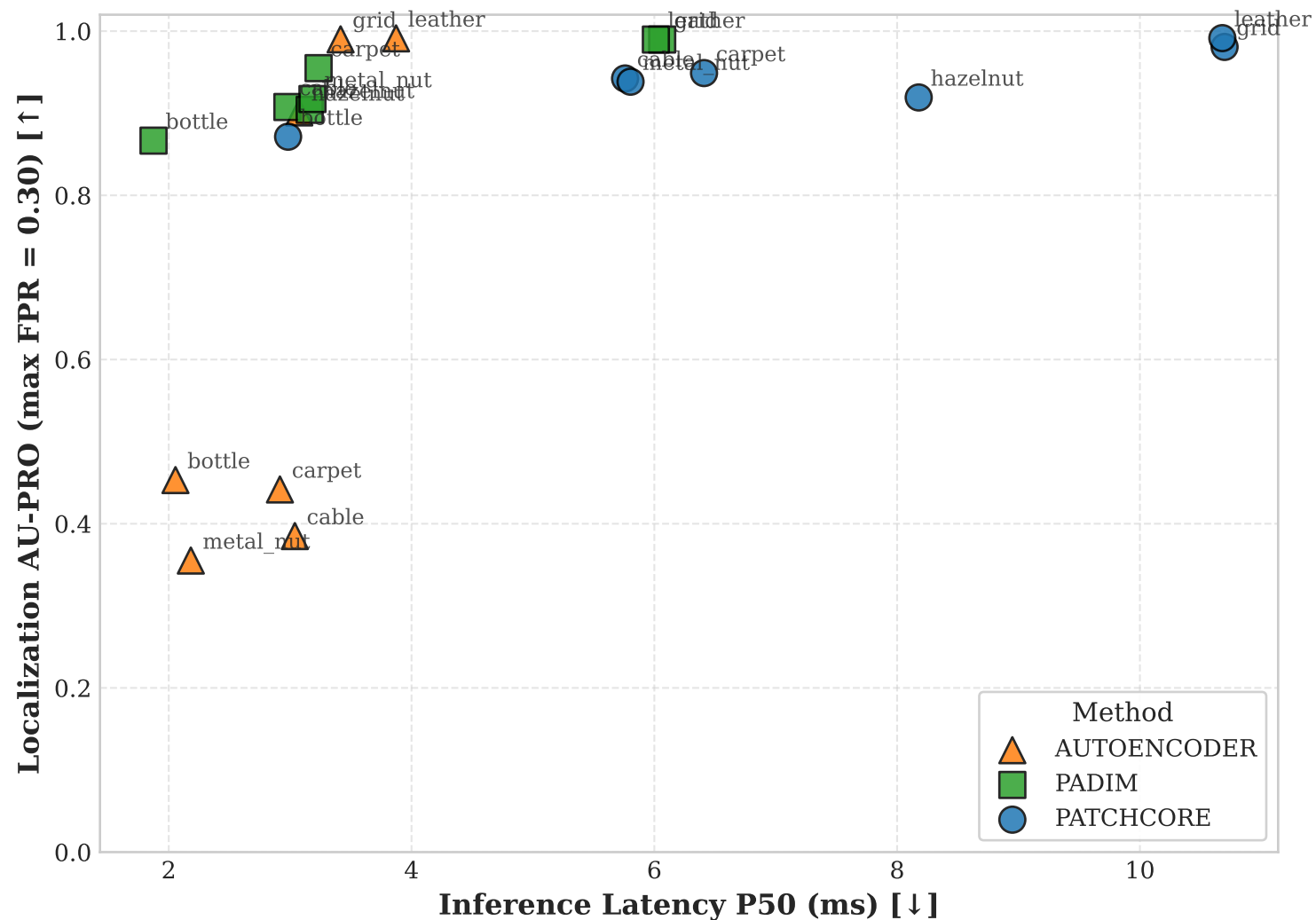
Pareto Frontier: Inference Speed vs. Defect Localization Accuracy
