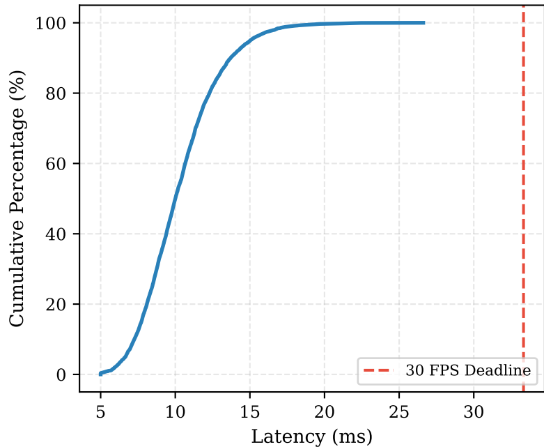
Deadline SLA Compliance (100% &lt;= 33.3ms)
