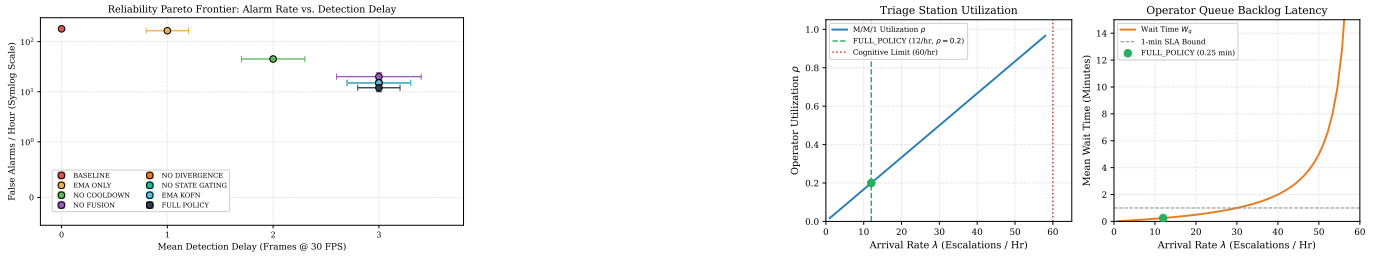
Fig. 1. Operational reliability and operator-workload analysis. (a) Trade-off between false alarm rate and mean detection delay across policy modes. (b) Operator-triage station utilization and expected wait time under M/M/1 queueing analysis. Shaded regions denote mathematically unstable queueing regimes ( \rho \geq 1.0 ) where review arrivals exceed operator triage capacity ( \mu = 60 reviews/hr).
