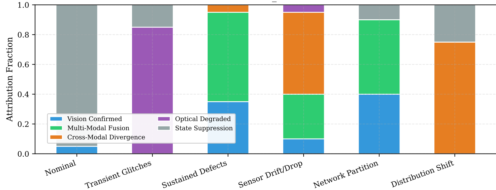
Decision Attribution for FULL_POLICY Across Workloads
