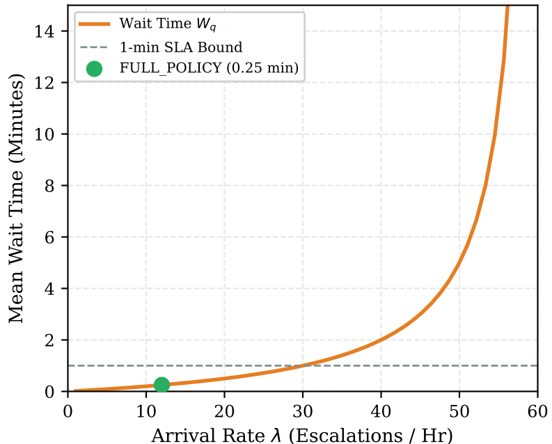
Operator Queue Backlog Latency
