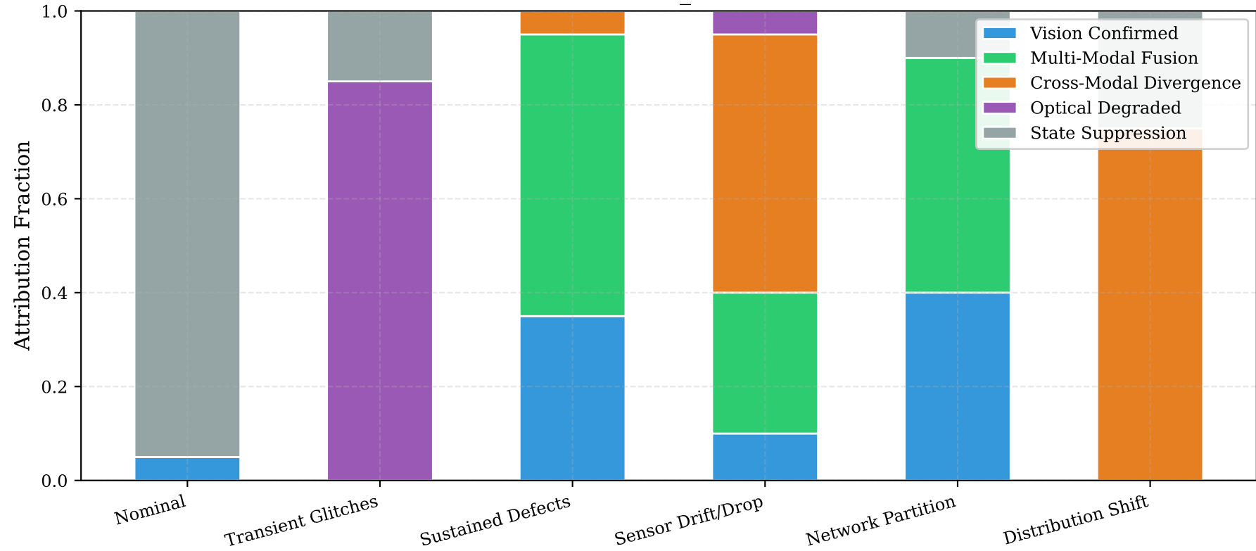
Granular Decision Attribution for FULL_POLICY Across Industrial Workloads
