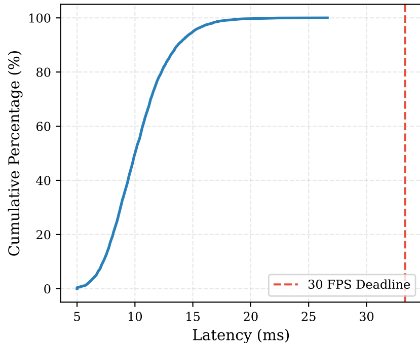
Deadline SLA Compliance (100% \leq 33.33ms)
