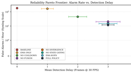
Fig. 1. Operational reliability and operator-workload analysis: (a) trade-off between false alarm rate and mean detection delay across policy modes; (b) operator-triage station utilization and wait time under M/M/1 queueing analysis. Shaded regions denote unstable queuing ( \rho \geq 1.0 ) exceeding operator triage capacity ( \mu = 60 reviews/hr).
