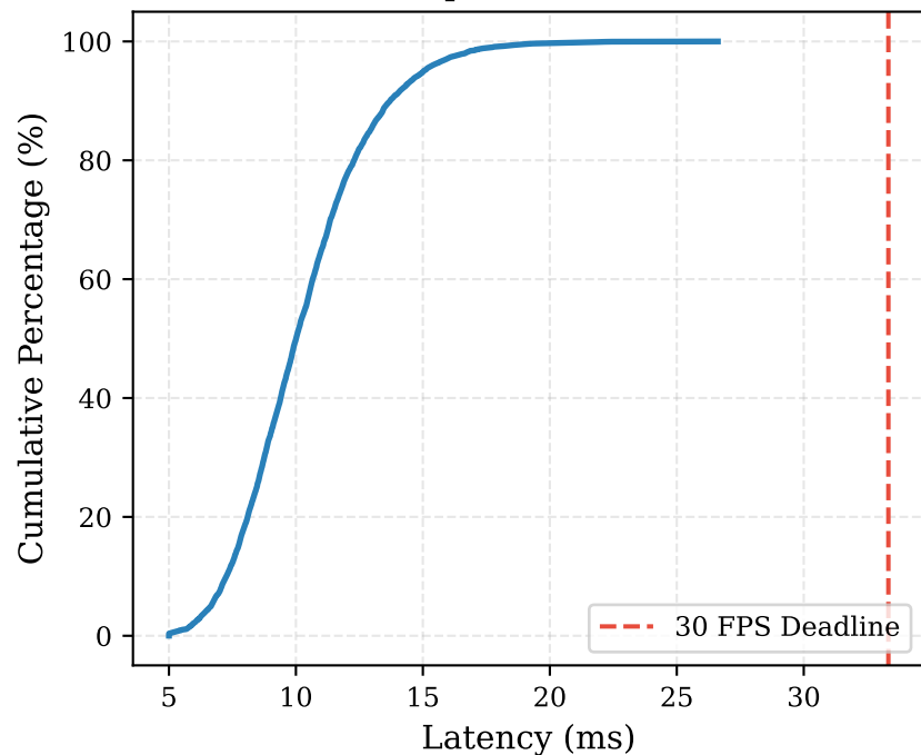
Deadline SLA Compliance (100% <= 33.33ms)
