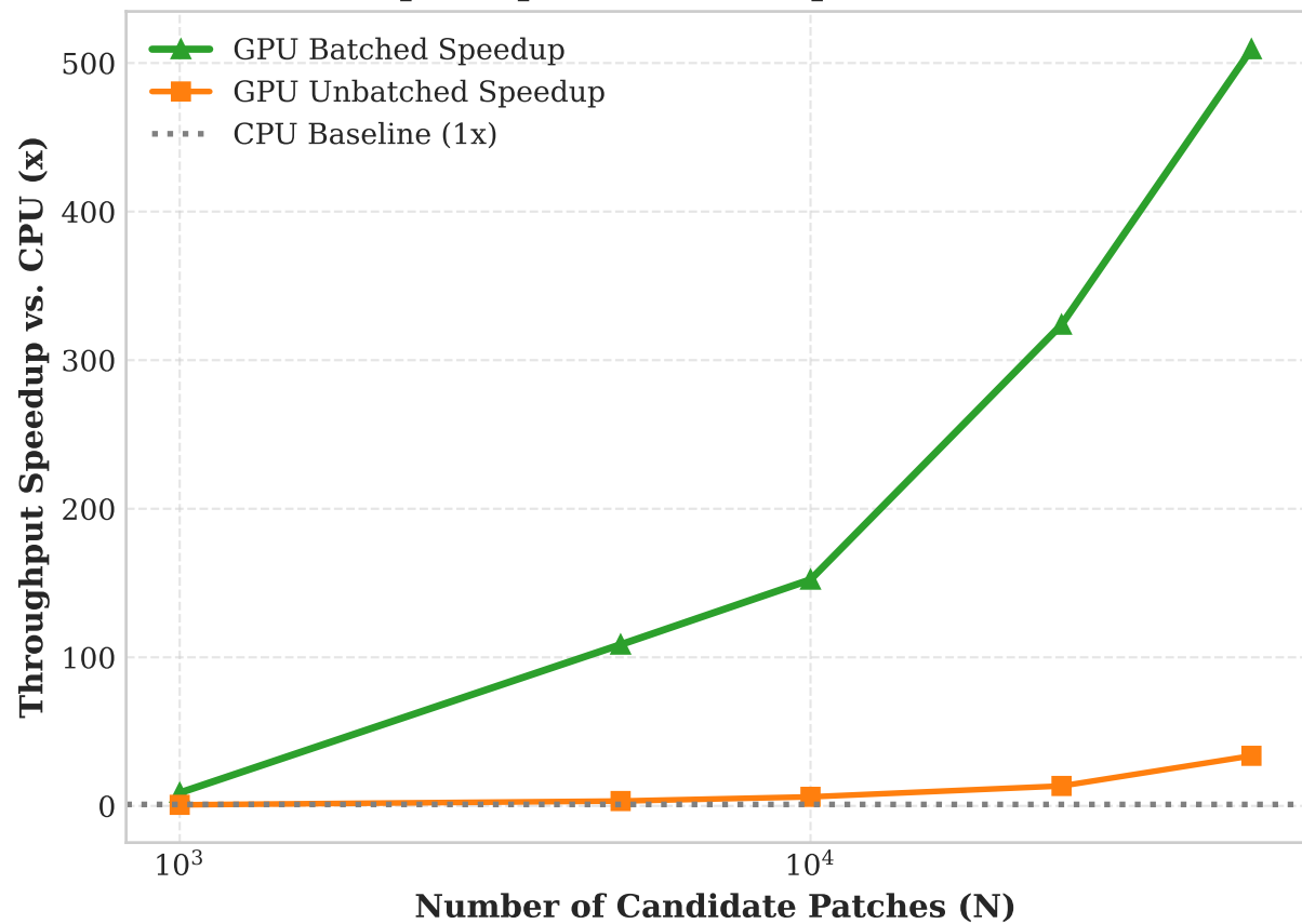
Speedup Factor vs. Sequential CPU
