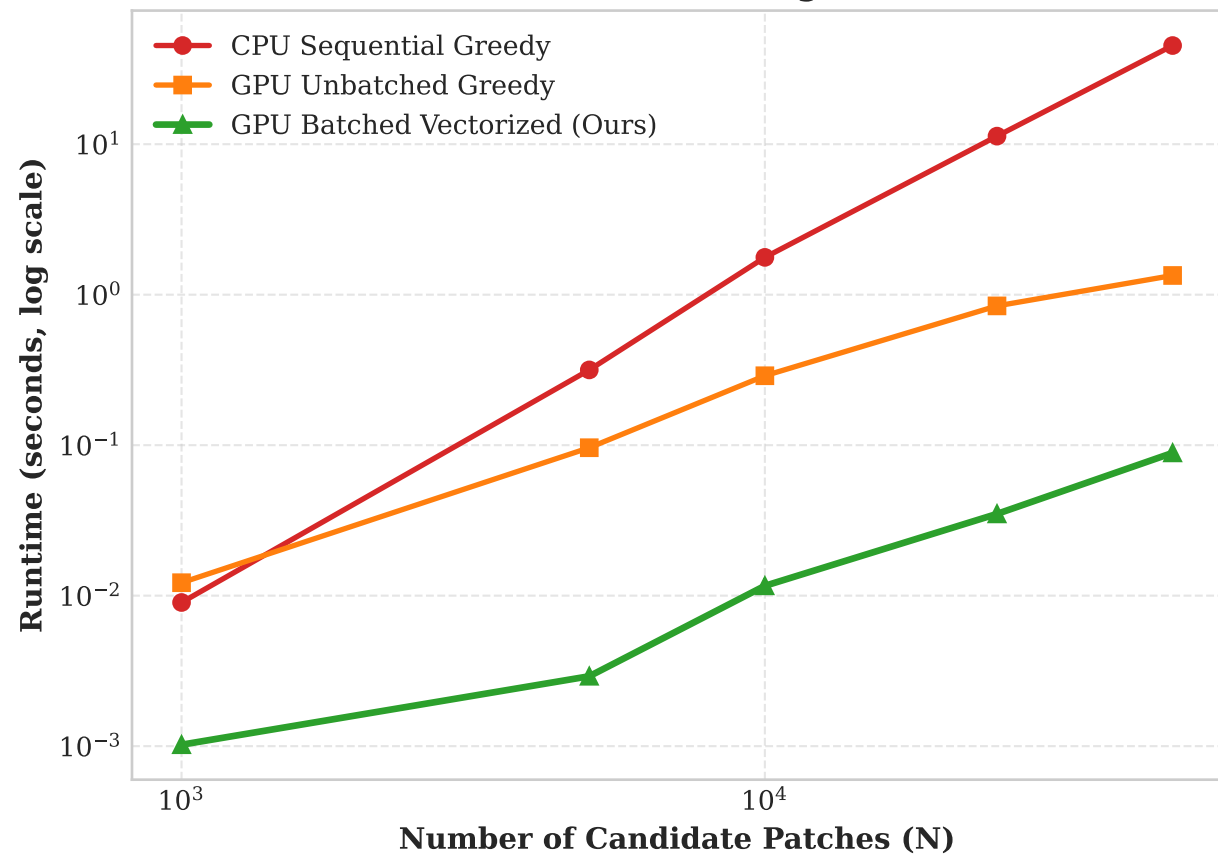
Coreset Runtime Scaling (D=128)
