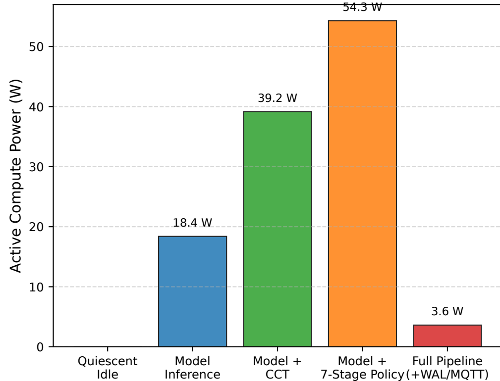
Active Hardware Power Draw on RTX 4050 GPU
