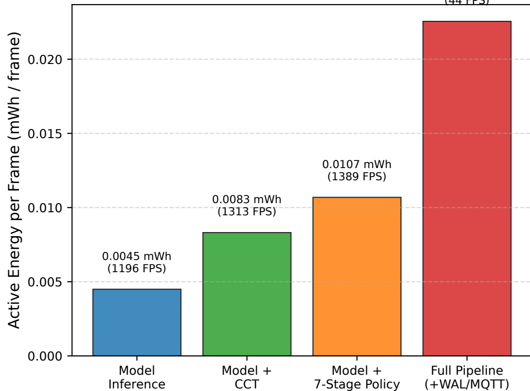
Energy Footprint per Inspected Frame
