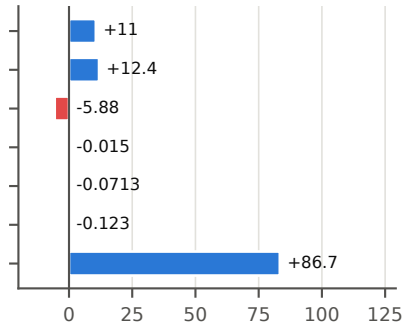
B: Machined metal: \Delta C = 104 \text{ kgCO}_2\text{e}
