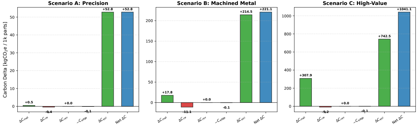
Fig. 6. Net carbon waterfall decomposition ( \Delta C = \Delta C_{\text{mat}} + \Delta C_{\text{rw}} + \Delta C_{\text{rev}} - C_{\text{edge}} + \Delta C_{\text{esc}} ) across Scenarios A, B, and C under Policy B4. Defect escape avoidance ( \Delta C_{\text{esc}} ) constitutes the primary positive contributor (scaling proportionally with embodied escape penalties across Scenarios A, B, and C), while continuous edge compute electricity ( -C_{\text{edge}} = -0.071 \text{ kgCO}_2\text{e} ) forms a persistent negative offset.
