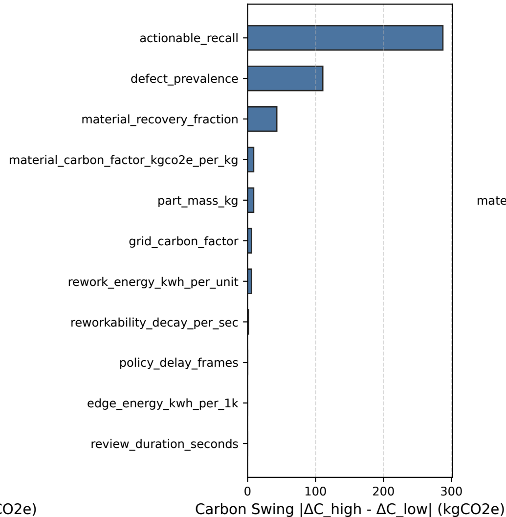
Scenario B: Machined Metal (Top Drivers)
