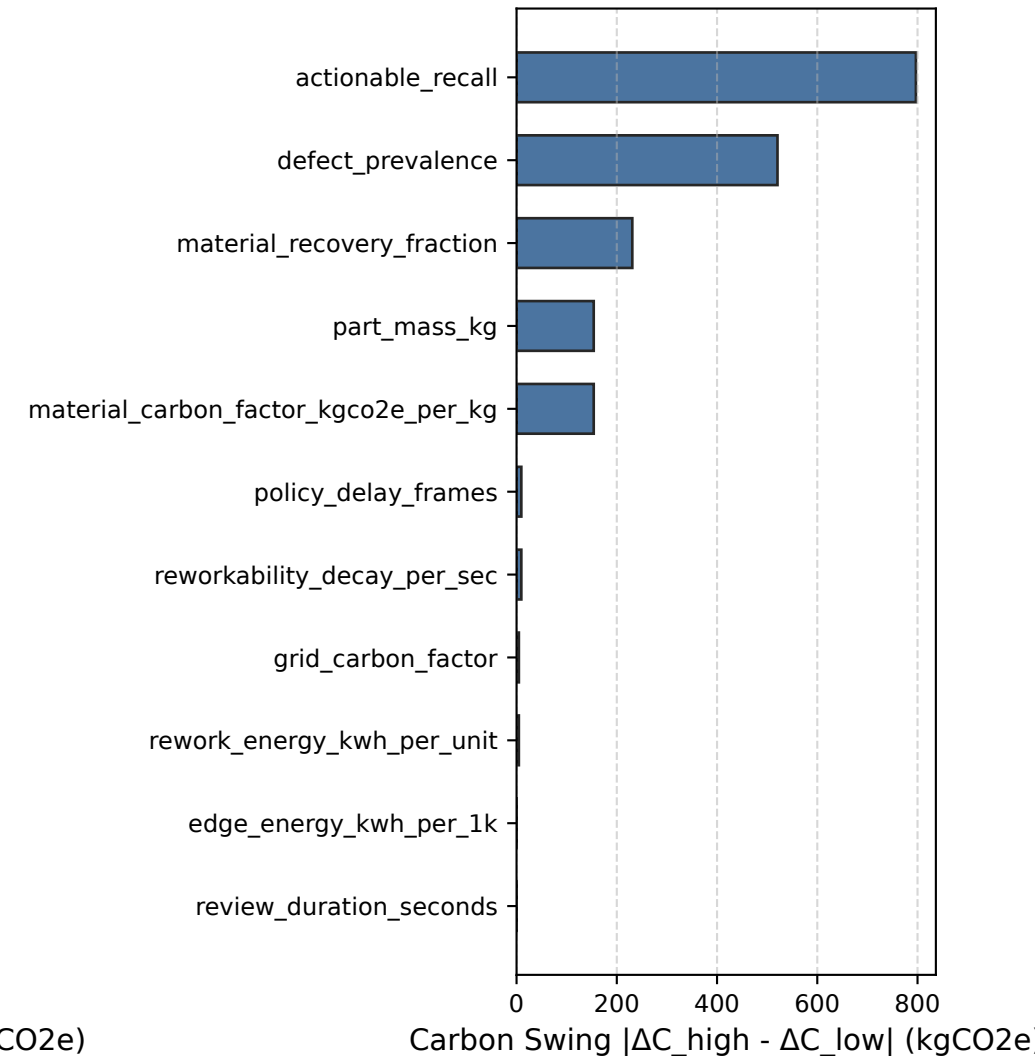
Scenario C: High Value (Top Drivers)
