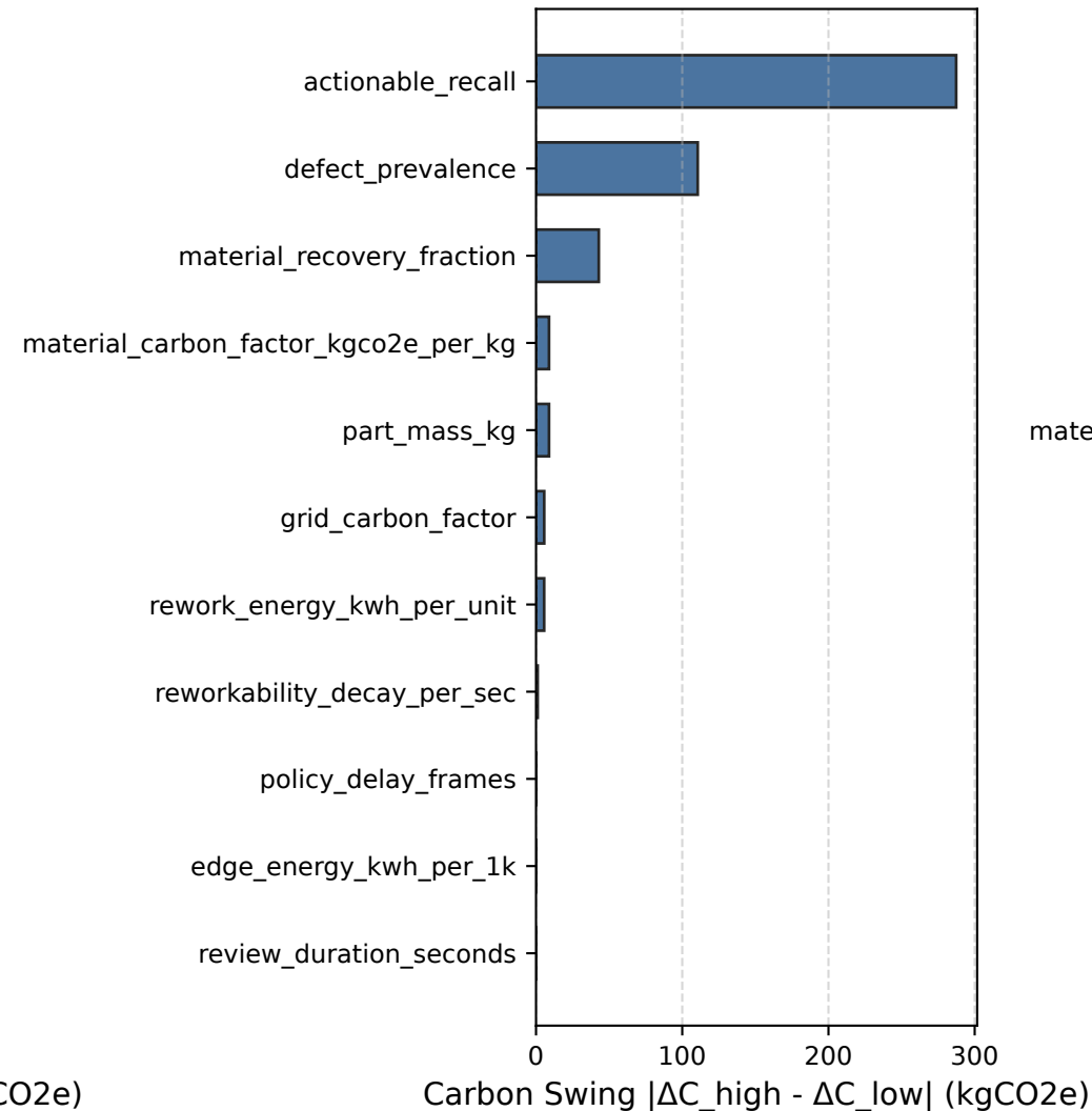
Scenario B: Machined Metal (Top Drivers)
