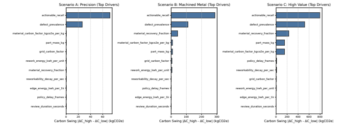
Fig. 4. Sensitivity and break-even frontiers across industrial scenarios. Left: 2D break-even heatmaps of net carbon benefit \Delta C across defect prevalence \pi and edge compute energy E_{\text{edge}} , illustrating the zero-carbon boundary ( \Delta C = 0 ). Right: 11-parameter tornado sensitivity rankings for \Delta C , demonstrating that actionable recall r_p and defect prevalence \pi are the dominant governing factors across all scenarios.
