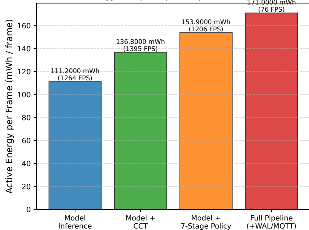
Energy Footprint per Inspected Frame
