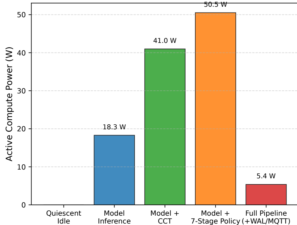
Active Hardware Power Draw on RTX 4050 GPU
