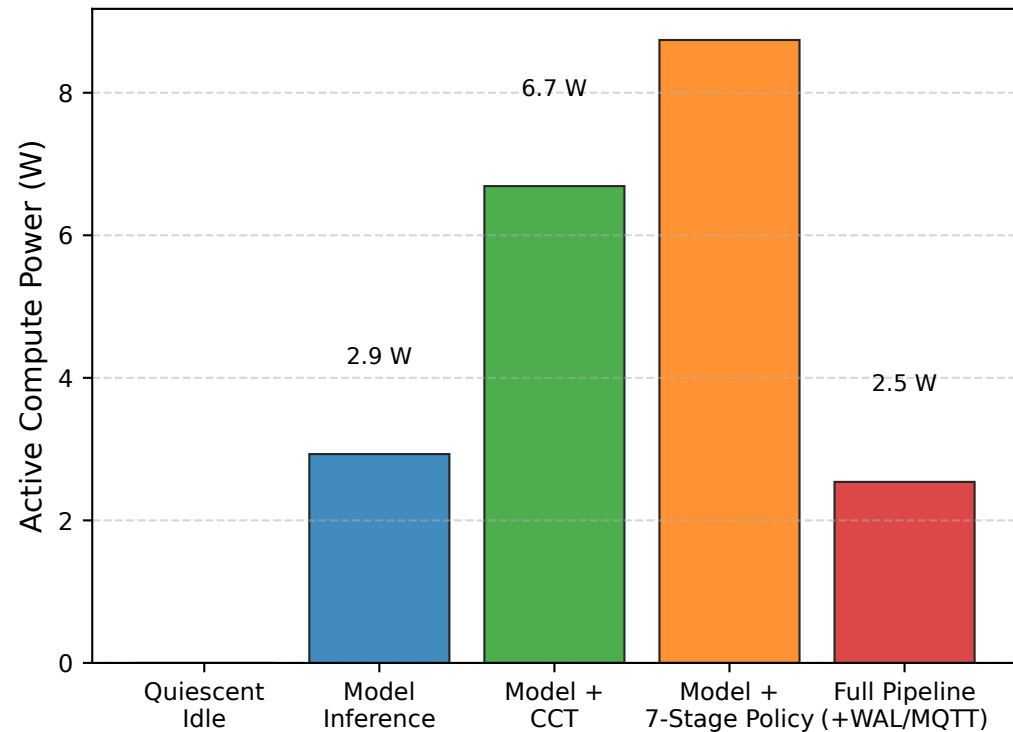
Active Hardware Power Draw on RTX 4050 GPU
