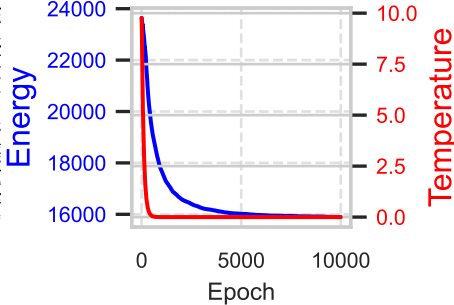
star - Energy/Temp
