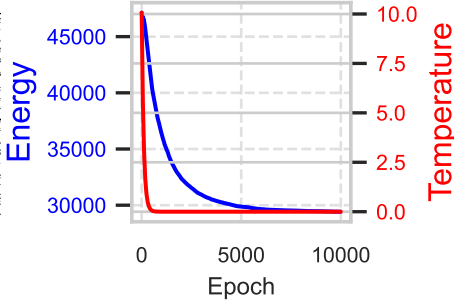
moore - Energy/Temp
