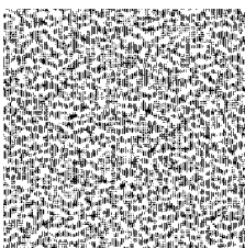
spiral - Grid
