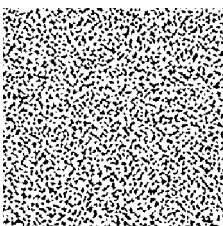
moore - Grid
