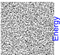
h - Grid
