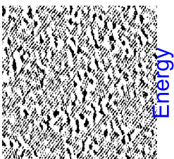
moss - Grid
