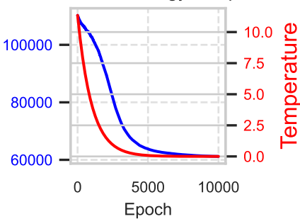
moore - Energy/Temp
