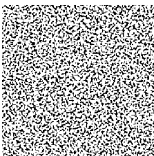
star - Grid
