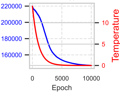
spiral - Energy/Temp
