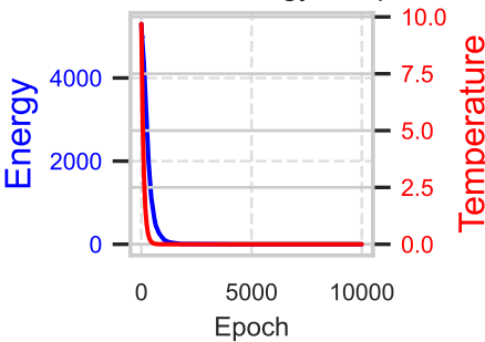
moore - Energy/Temp
