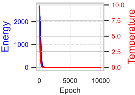
star - Energy/Temp
