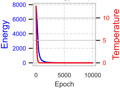
h - Energy/Temp
