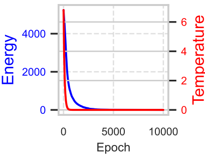
staircase - Energy/Temp
