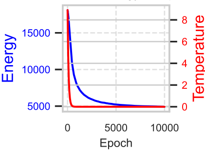
moss - Energy/Temp
