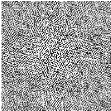
staircase - Grid
