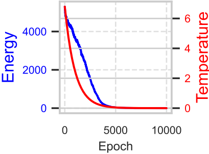
staircase - Energy/Temp
