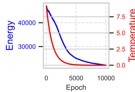
staircase - Energy/Temp
