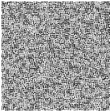
spiral - Grid
