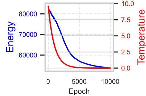
staircase - Energy/Temp
