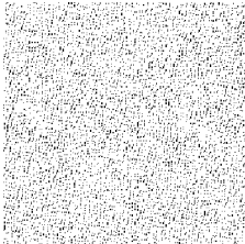
h - Grid
