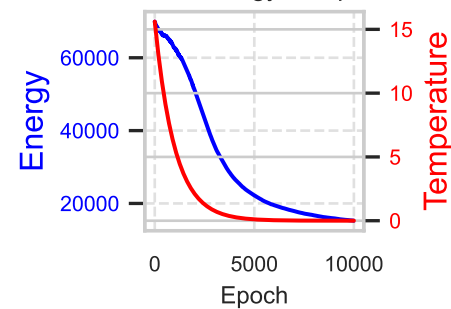
h - Energy/Temp
