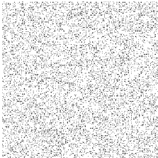
moore - Grid
