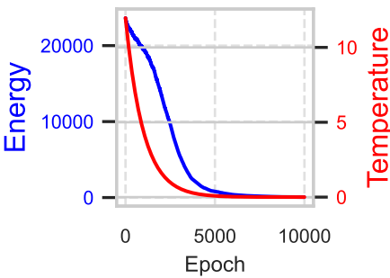
star - Energy/Temp
