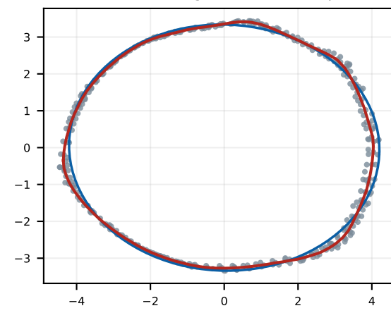
h 10 4 → N6 / T12 girth 25.5 mesh/pts 0.99
