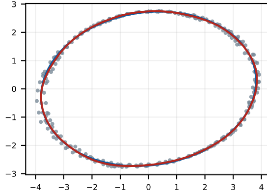
h 0 4 → sphere 16 girth 20.7 mesh/pts 1.00
