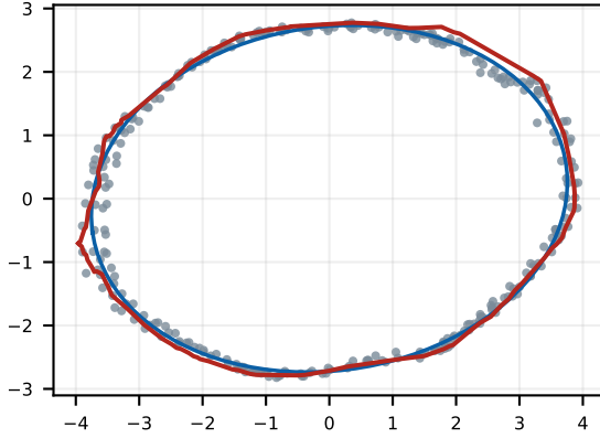
h 0 today girth 20.5 mesh/pts 1.04
