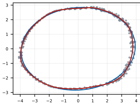
h 4 4 → N6 / T12 girth 21.4 mesh/pts 0.99
