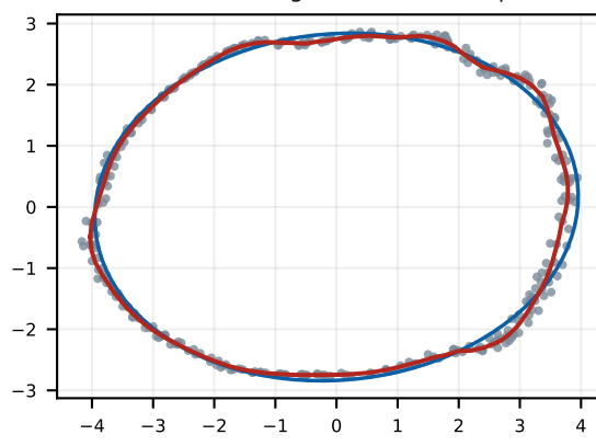
h 4 4 → N12 / T6 girth 21.5 mesh/pts 0.99
