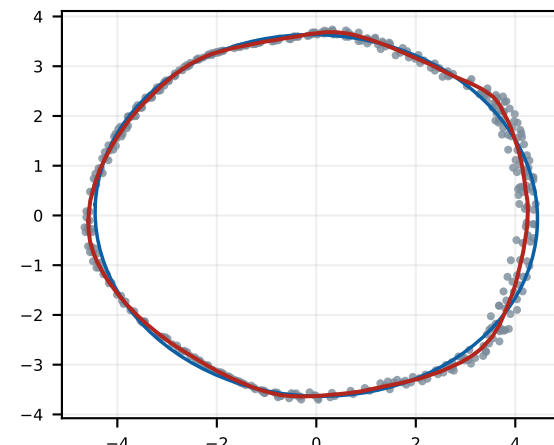
h 12 4 → N6 / T12 girth 27.3 mesh/pts 0.99
