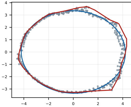
h 10 today girth 25.5 mesh/pts 1.06
