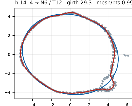
h 14 4 → N6 / T12 girth 29.3 mesh/pts 0.99
