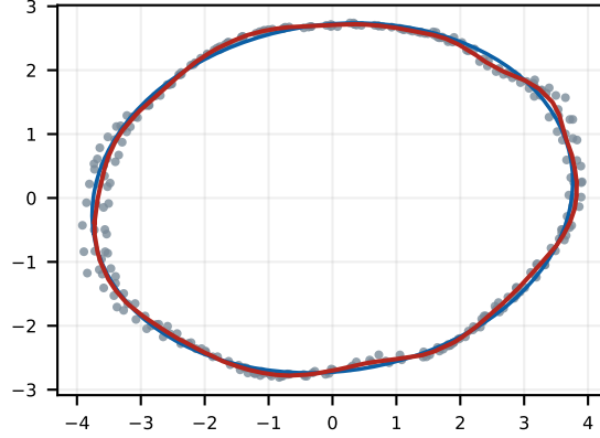
h 0 4 → N12 / T6 girth 20.5 mesh/pts 0.99
