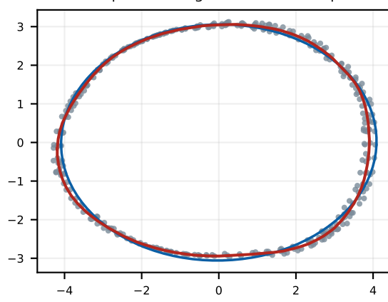
h 6 4 → sphere 16 girth 22.6 mesh/pts 0.99
