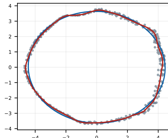
h 12 4 → N12 / T6 girth 27.3 mesh/pts 0.98
