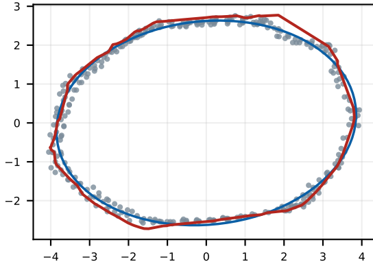
h 2 today girth 20.5 mesh/pts 1.05
