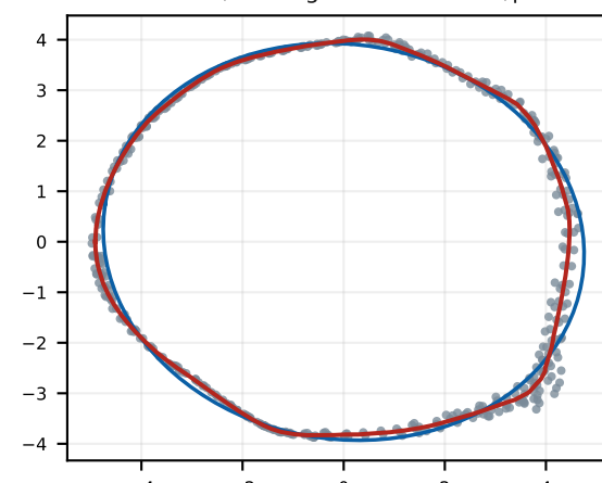
h 14 4 → N6 / T12 girth 29.3 mesh/pts 0.99
