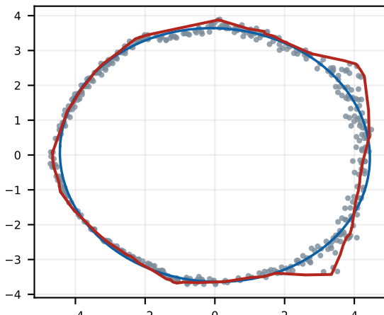
h 12 today girth 27.4 mesh/pts 1.08
