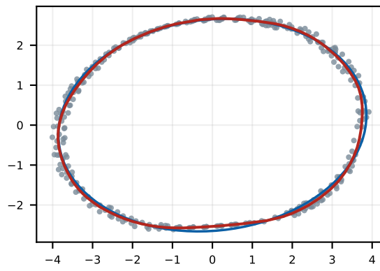
h 2 4 → sphere 16 girth 20.6 mesh/pts 0.99
