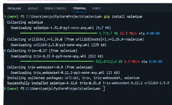
Figure 5: Install Selenium
