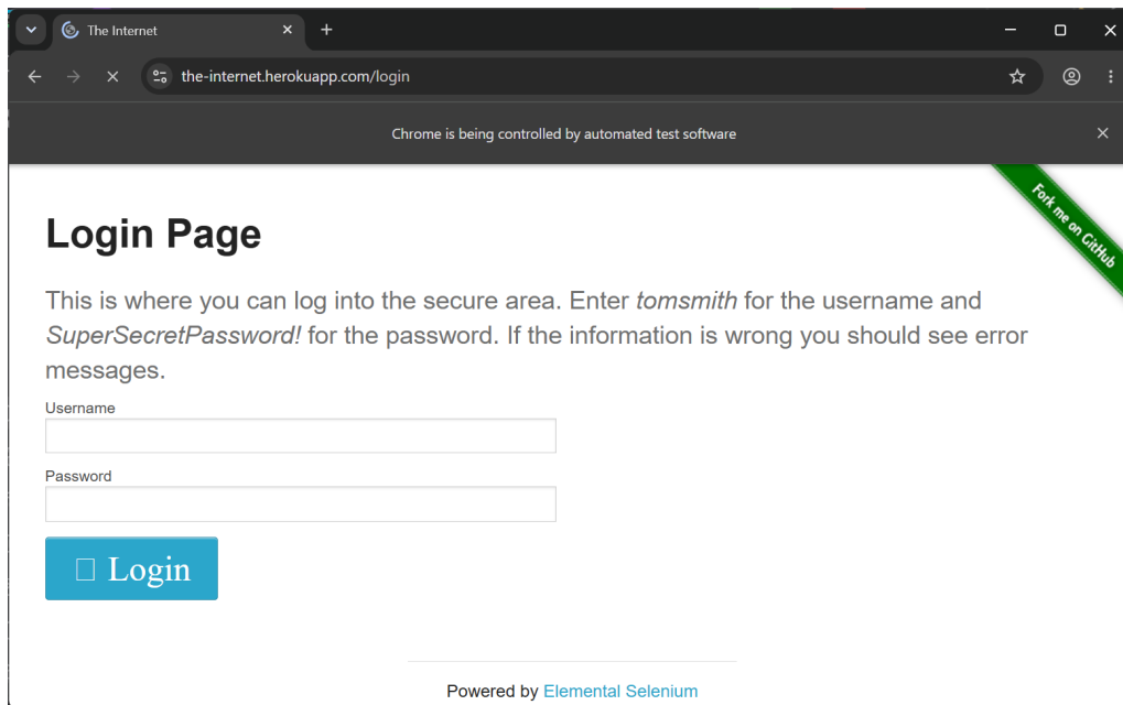
Figure 14: execution evidence
