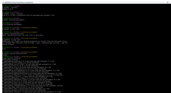
Figure 3: Enter Caption
