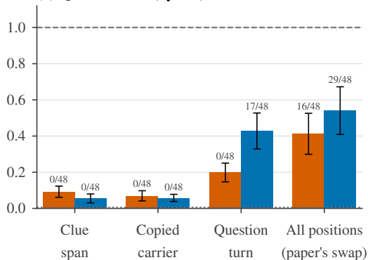
(a) Qwen3.6-27B (hybrid)
