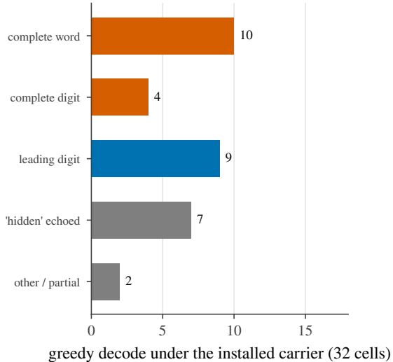
(b) Greedy decode
