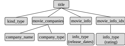
Fig. 15: Join tree of the JOB 13d acyclic core.
