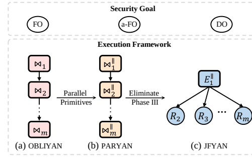
Fig. 1: Different ways of handling Phase III under different obliviousness goals.
