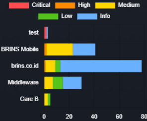
Vulnerability Severity by Asset
