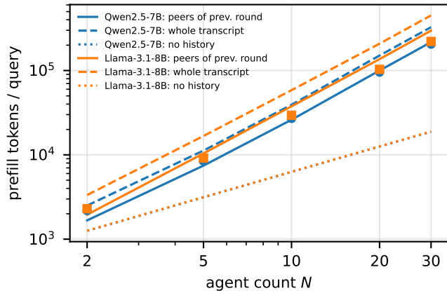
(b) which transcript an agent re-reads
