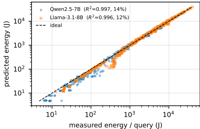
(a) two-rate model vs measurement
