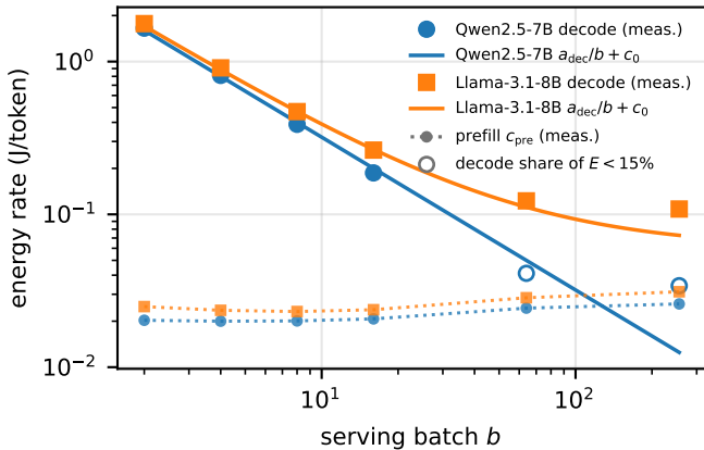
(b) decode \sim 1/b , prefill flat
