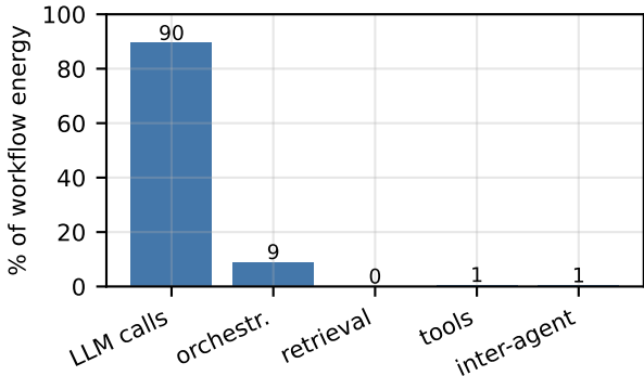
Llama-3.1-8B coefficients, b=64
