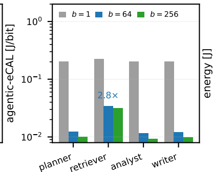
(c) energy per useful bit
