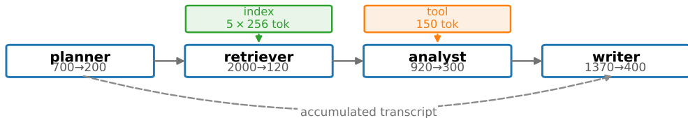
(a) the four-agent RAG workflow
