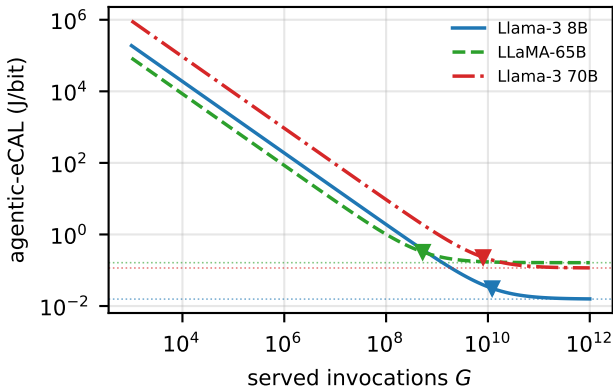
Amortization (NVIDIA A100 80GB, b=64 )
