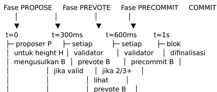
Gambar 2 — Timing ronde BFT
