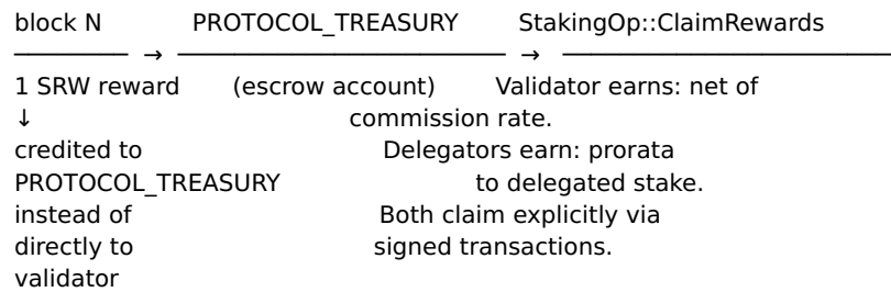
Figure 4 — Reward routing
