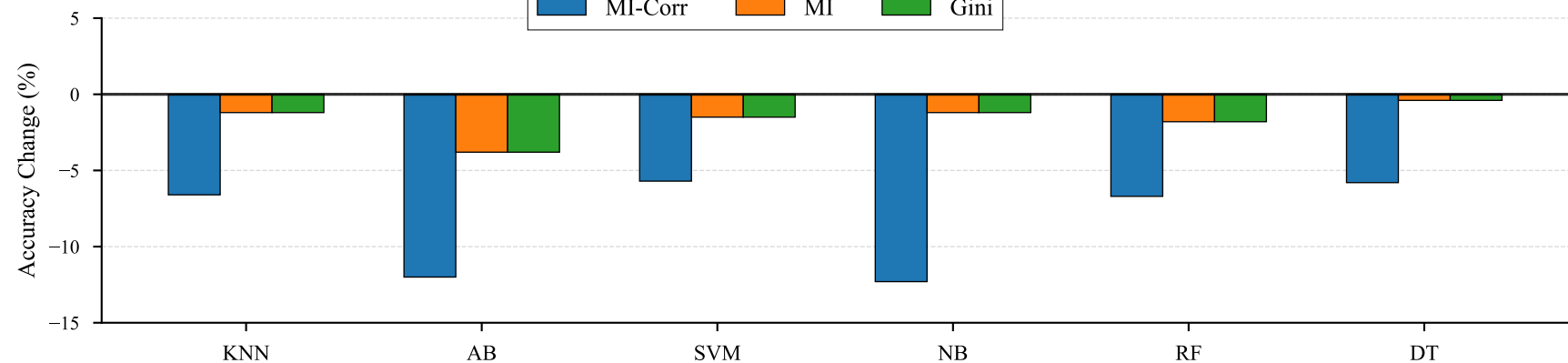
Divorce Dataset
