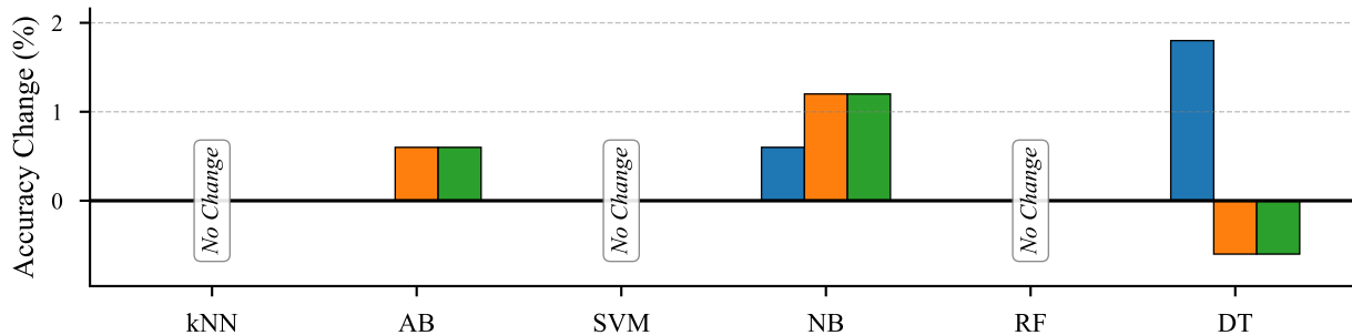
Parkinsons Dataset
