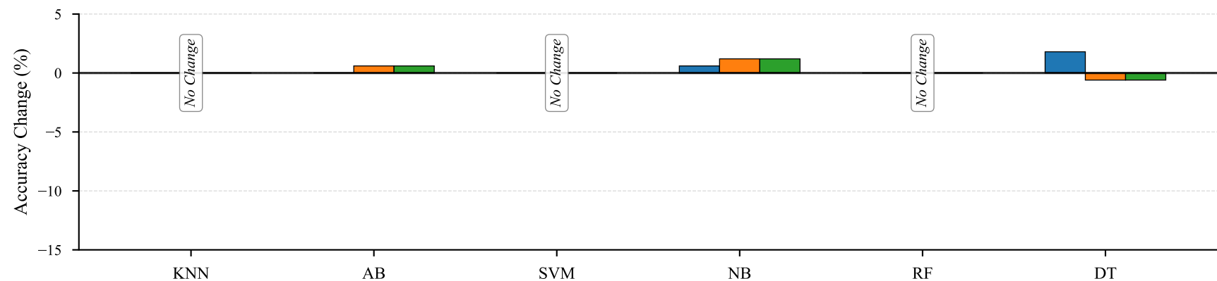
Parkinsons Dataset
