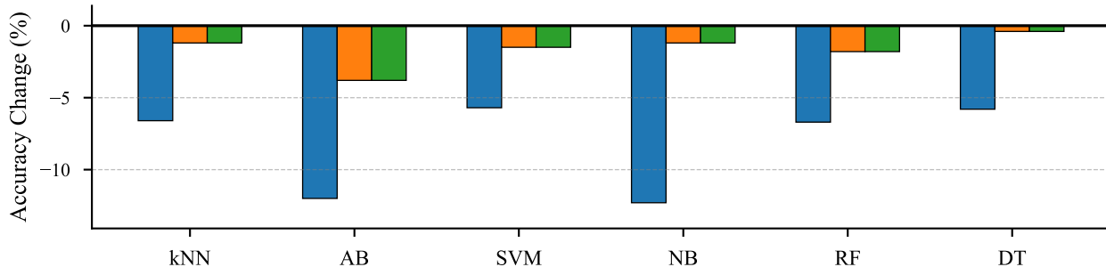
Divorce Dataset
