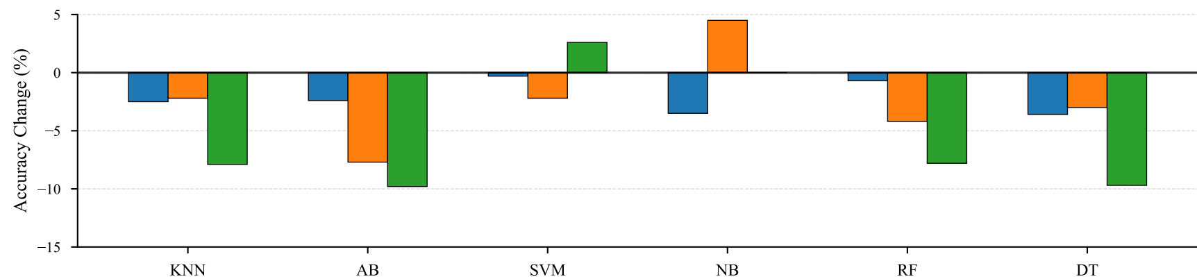
Rice Dataset
