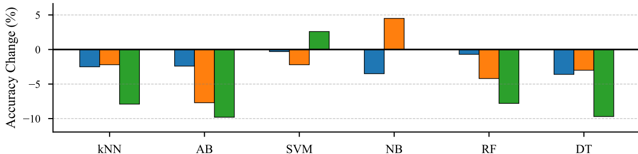
Rice Dataset
