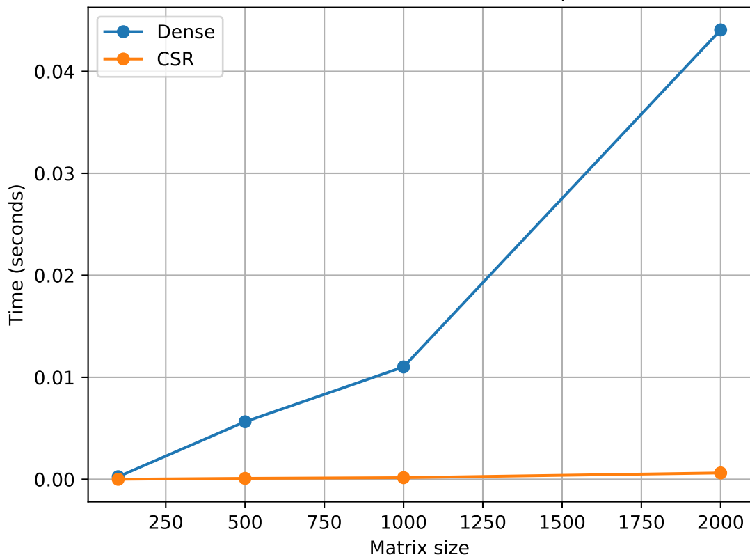
Dense vs CSR matrix-vector multiplication
