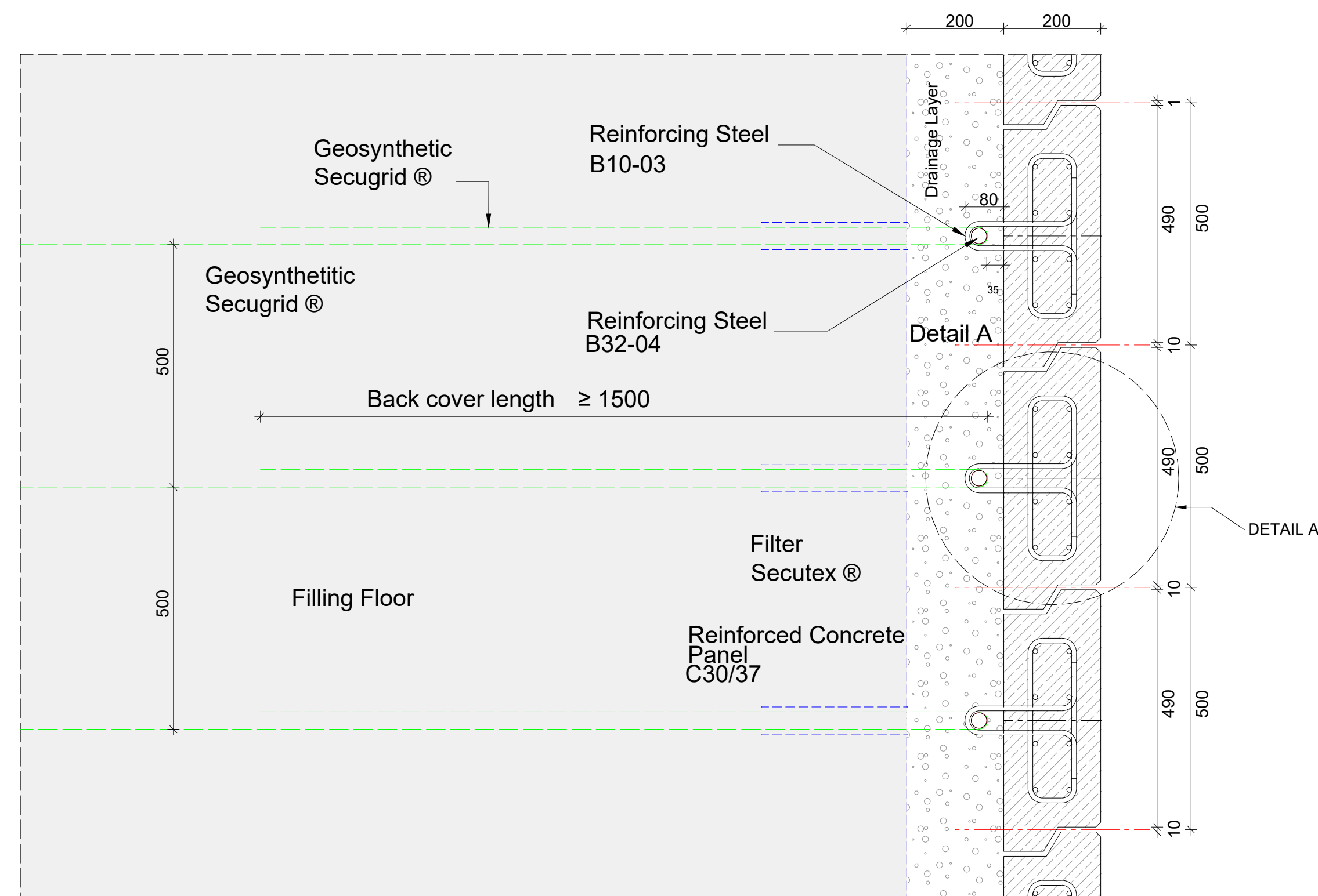
SECTION 2 - 2 REBAR DETAILS
