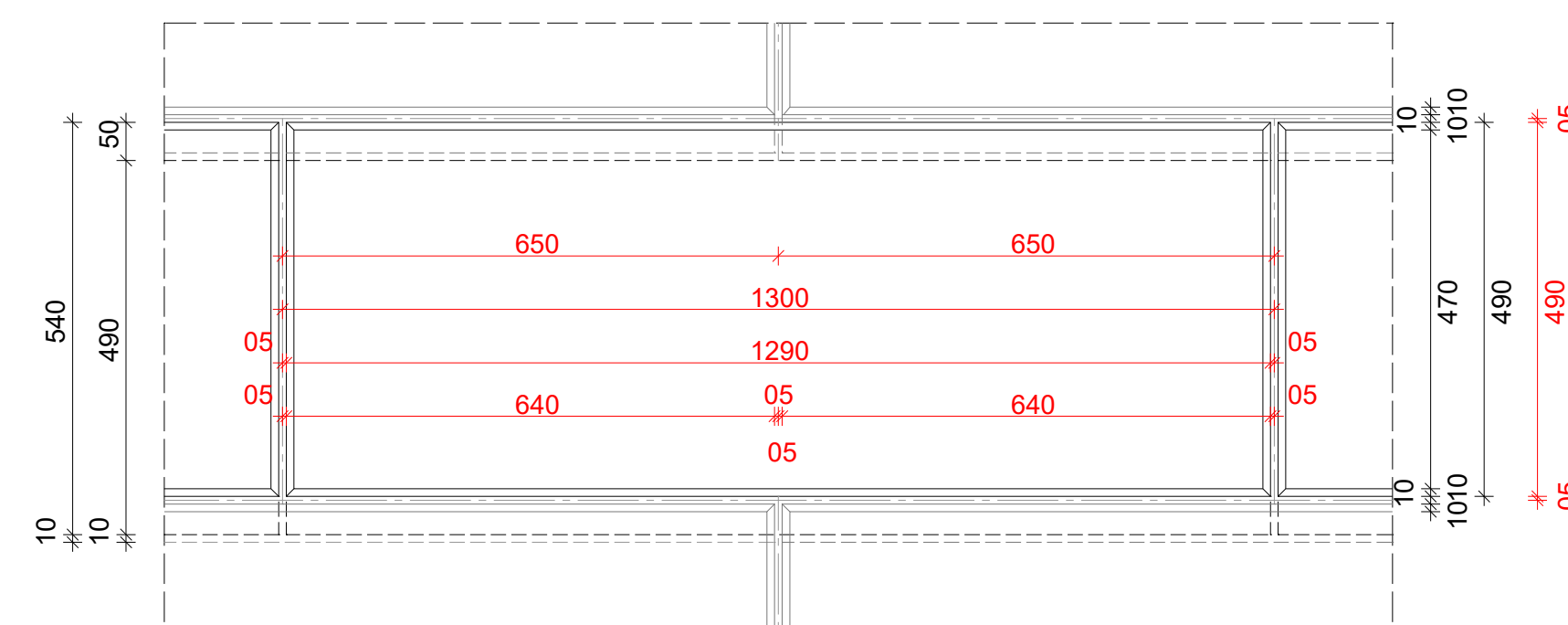
DETAIL A FRONT VIEW
