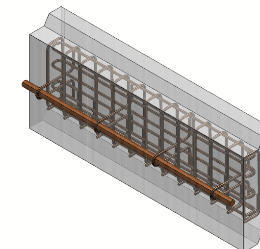
3D VIEW DRAWN NOT TO SCALE
