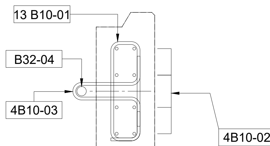
SECTION 2 - 2 REBAR DETAILS
