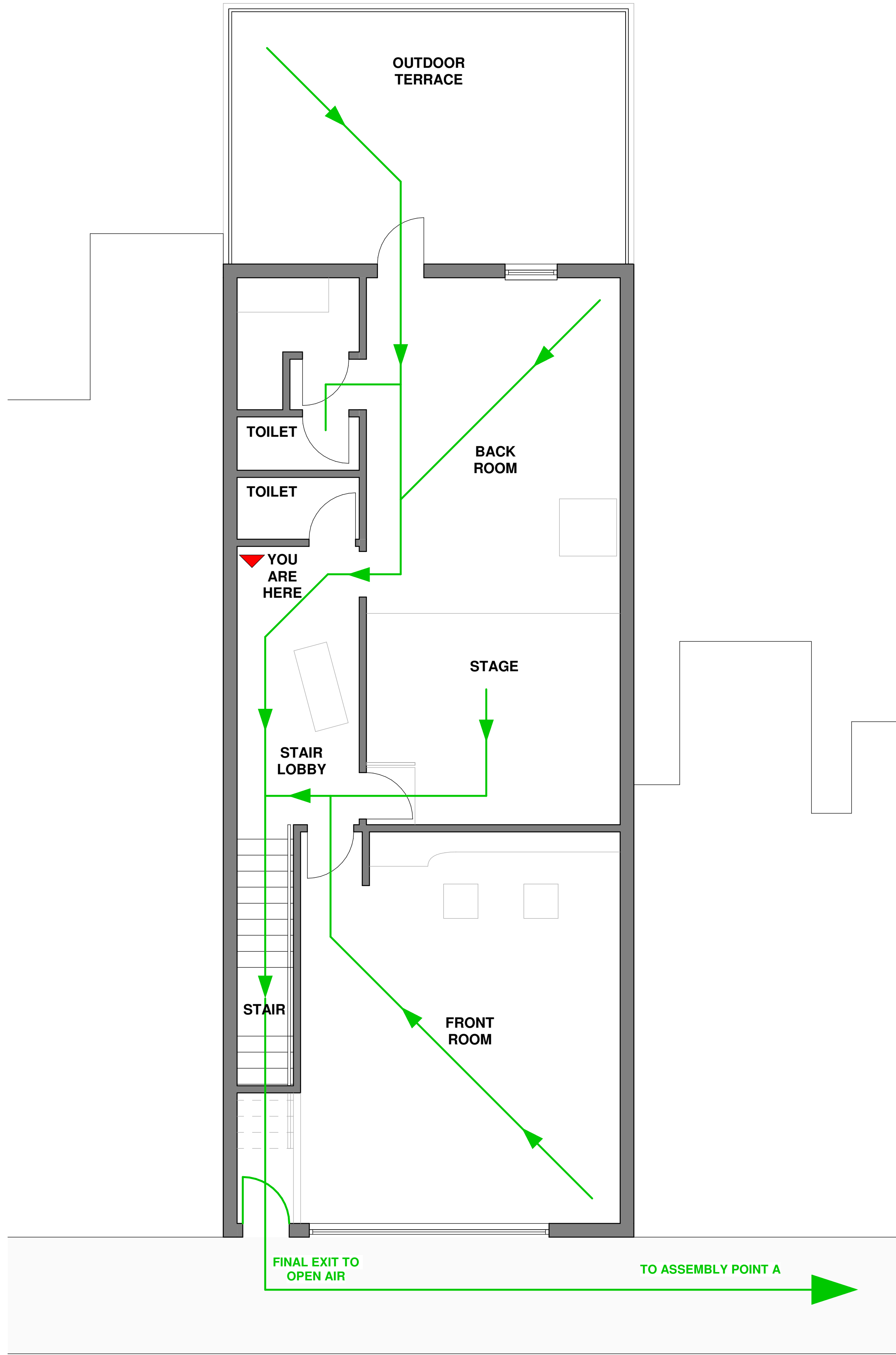
NCF - FIRST FLOOR PLAN
