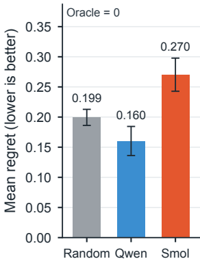
(a) Selection regret
