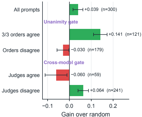
(b) Gain over random: kept vs. rejected
