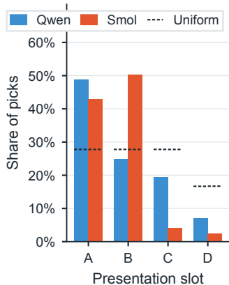
(c) Presentation-slot preference
