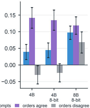
(b) Gain over random
