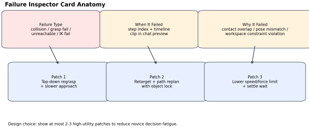
Figure 2: Failure Inspector structure in ArmCraft: what failed, when it failed, why it failed, and a short patch set for immediate re-simulation.
