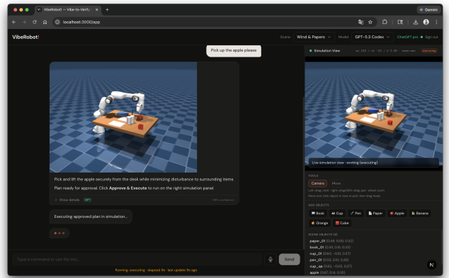
Figure 4: Runtime walkthrough (Part I, left-to-right/top-to-bottom): S0 onboarding and scene setup, S1 command entry, S2 reasoning + simulation preview, and S3 explicit approval gate ( Reject vs Approve & Execute ).
