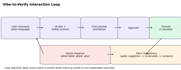
Figure 3: Vibe-to-Verify interaction loop. The user remains in control through explicit approval and patch-guided repair.
