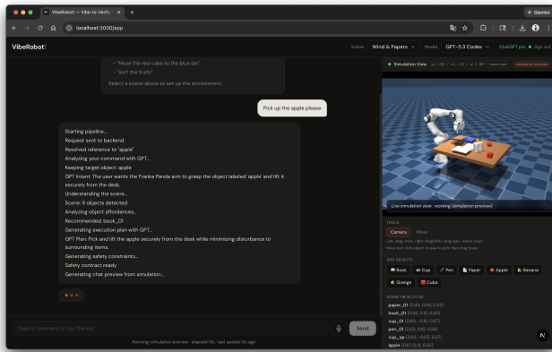
Figure 4: Runtime walkthrough (Part I, left-to-right/top-to-bottom): S0 onboarding and scene setup, S1 command entry, S2 reasoning + simulation preview, and S3 explicit approval gate ( Reject vs Approve & Execute ).
