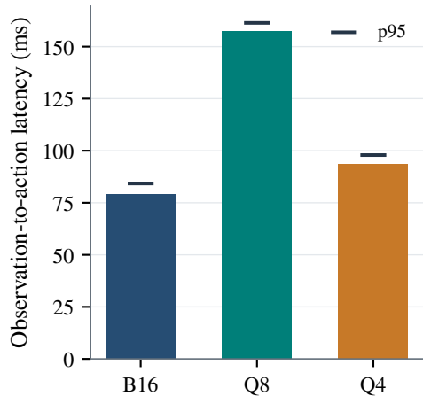
a Inference time
