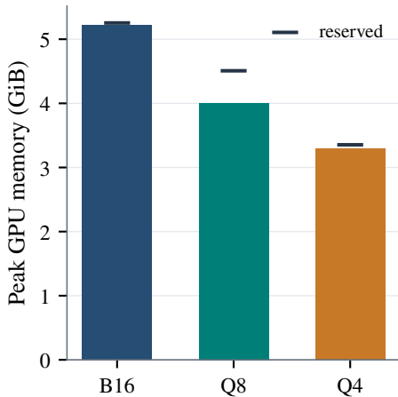
b Inference footprint
