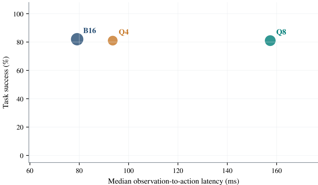
RTX 3090 · development · bubble area \propto peak allocated VRAM
