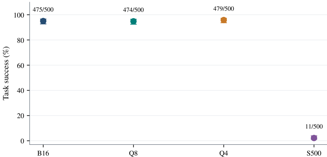
LIBERO-Spatial · final · 95% Wilson intervals
