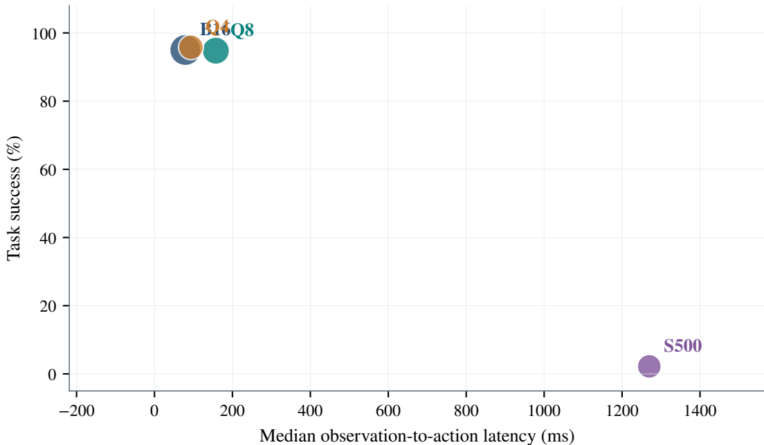
RTX 3090 · final · bubble area \propto peak allocated VRAM
